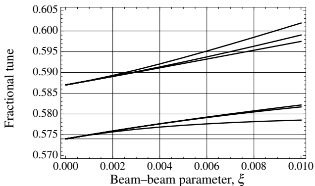
Figure 1: Coherent mode tunes versus the beam–beam parameter per IP, calculated with the linearized model; here Q_p = 0.587 , Q_a = 0.574 , and \xi = \xi_p = \xi_a .
